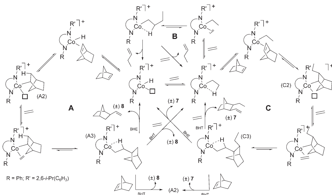
Scheme 9. Possible mechanistic paths for the 2E-1NB hetero-trimerization reaction.
