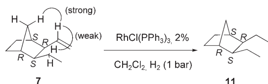
Figure 2. NOE effect on 7 and catalytic hydrogenation to 11 .
