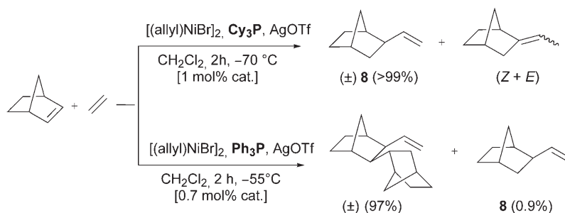
Scheme 2. Phosphine ligand dependence in the NB hydrovinylation.
