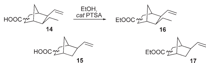
Scheme 6. Esterification of the crude acid mixture.
