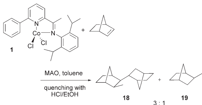
Scheme 8. Stoichiometric reaction of 1 with NB.
