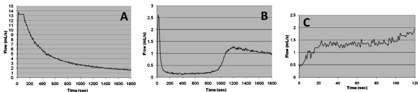
Figure 3. A ) E consumption in E oligomerization ( 1 , 12 \mu\text{mol} ; E, 4 bar; toluene, 100 mL; MAO, 600 equiv; 30 min; 25 °C); B ) E/NB co-oligomerization (Table 1, entry 4); C ) E/NB co-oligomerization (Table 1, entry 18).
