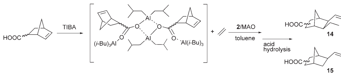
Scheme 5. E/TIBA-protected NB COOH Co-catalyzed hetero-trimerization.
