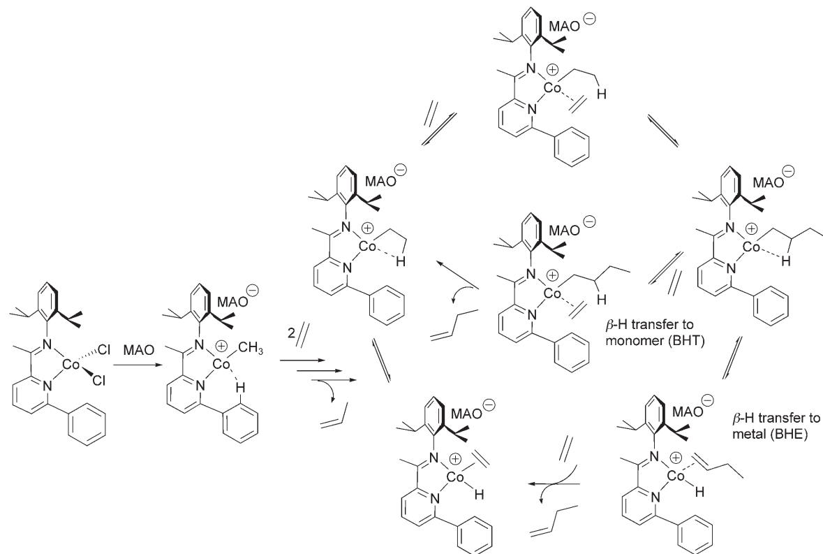
Scheme 7. Reaction paths for the dimerization of E catalyzed by 1 /MAO.
