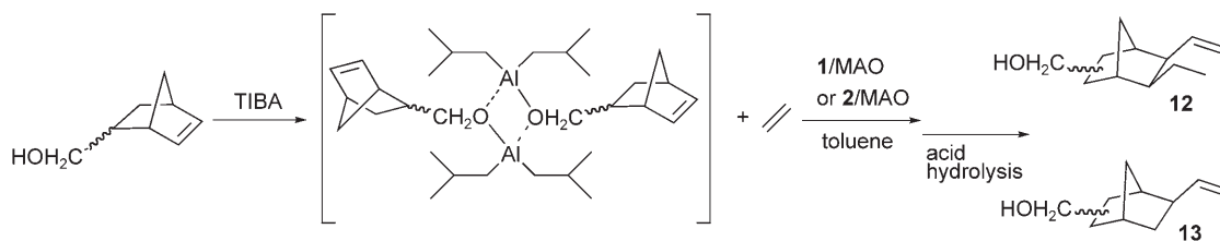
Scheme 4. E/TIBA-protected NB OH Co-catalyzed hetero-trimerization.
