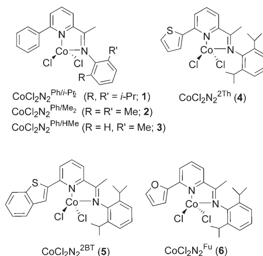
Figure 1. \text{CoCl}_2 (imino)pyridine pre-catalysts for olefin oligomerization.
