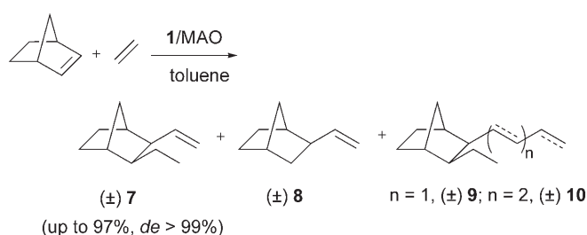
Scheme 1. 1/MAO catalyzed 2E-1NB hetero-trimerization.
