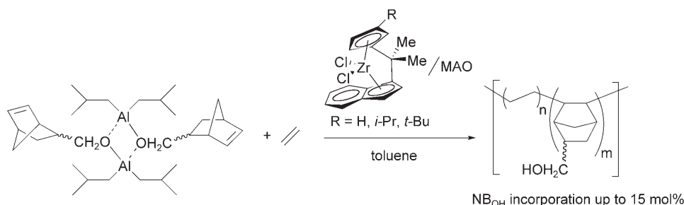
Scheme 3. E/TIBA-protected NB OH copolymerization by a metallocene/MAO system.
